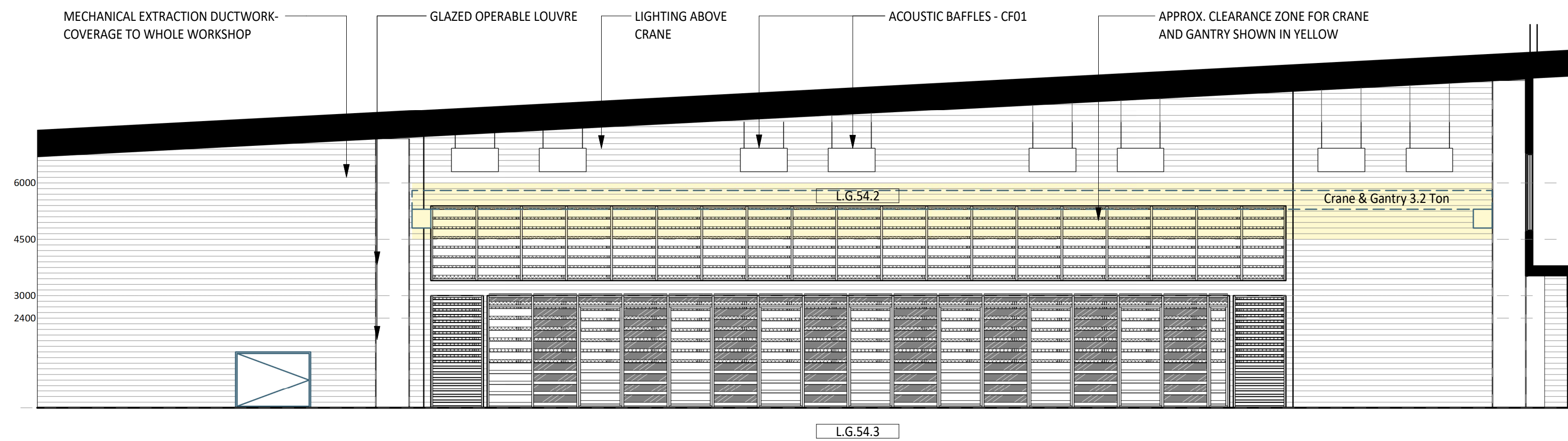
4 ELEVATION DETAIL 60-001 1 : 100
