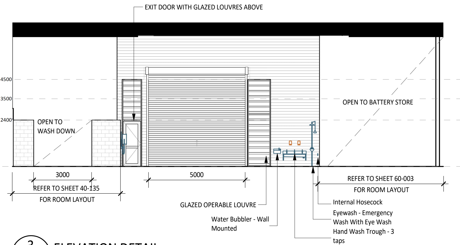
3 ELEVATION DETAIL 60-001 1 : 100
