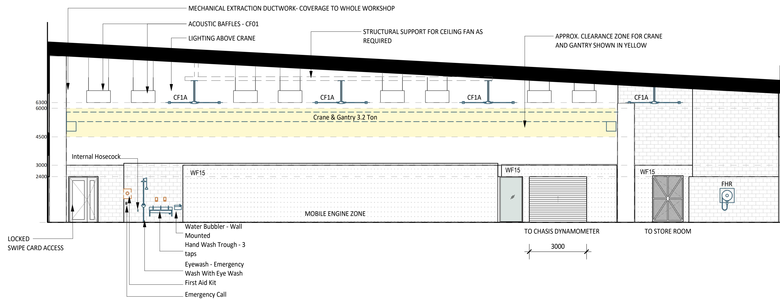
2 ELEVATION DETAIL 60-001 1 : 100
